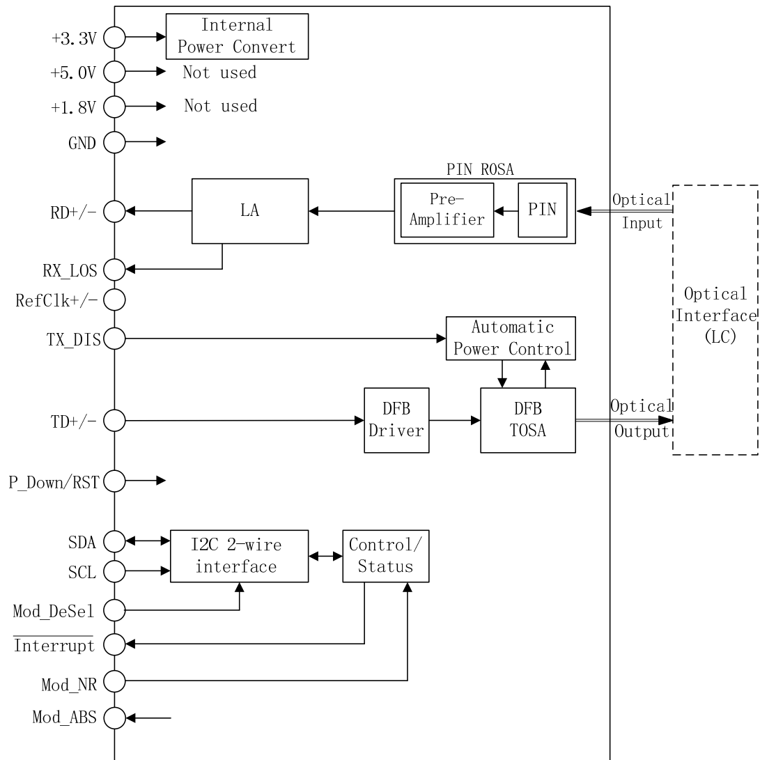
Figure 1. 40km 2.5Gb/s SFP internal structure
